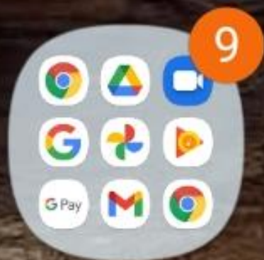
Google
