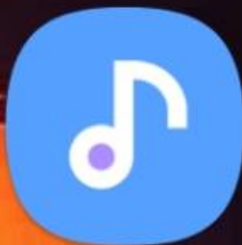
Samsung Music
