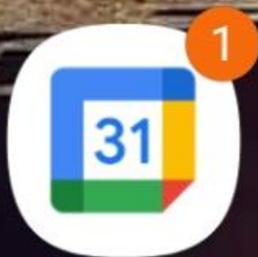
Calendar
