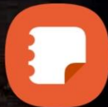
Samsung Notes
